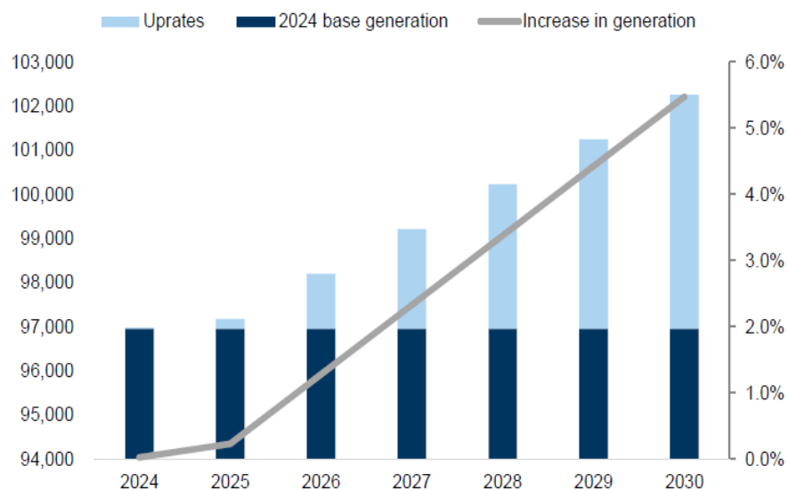
Nuclear uprated impact on nuclear power generation
