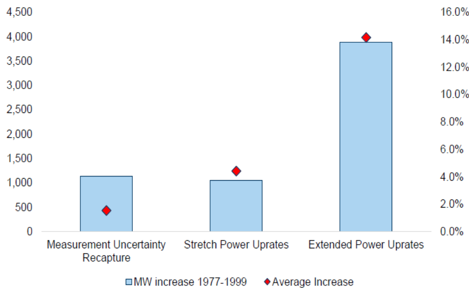
MW additions by type of power uprates
